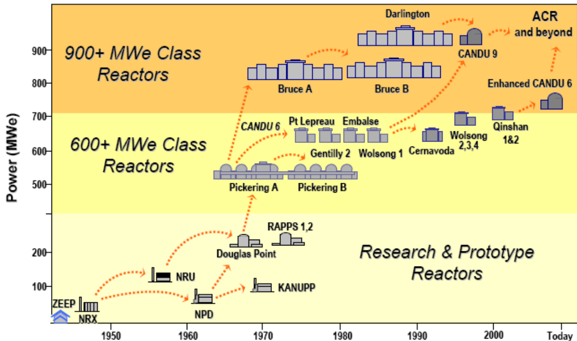
Figure 3: CANDU Genealogy
